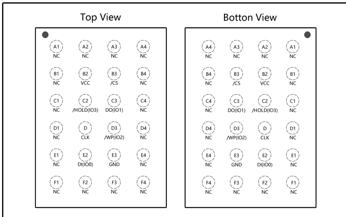
Figure 1e. UD25Q128A Ball Assignments, 24-ball WLCSP (Package Code Y)
