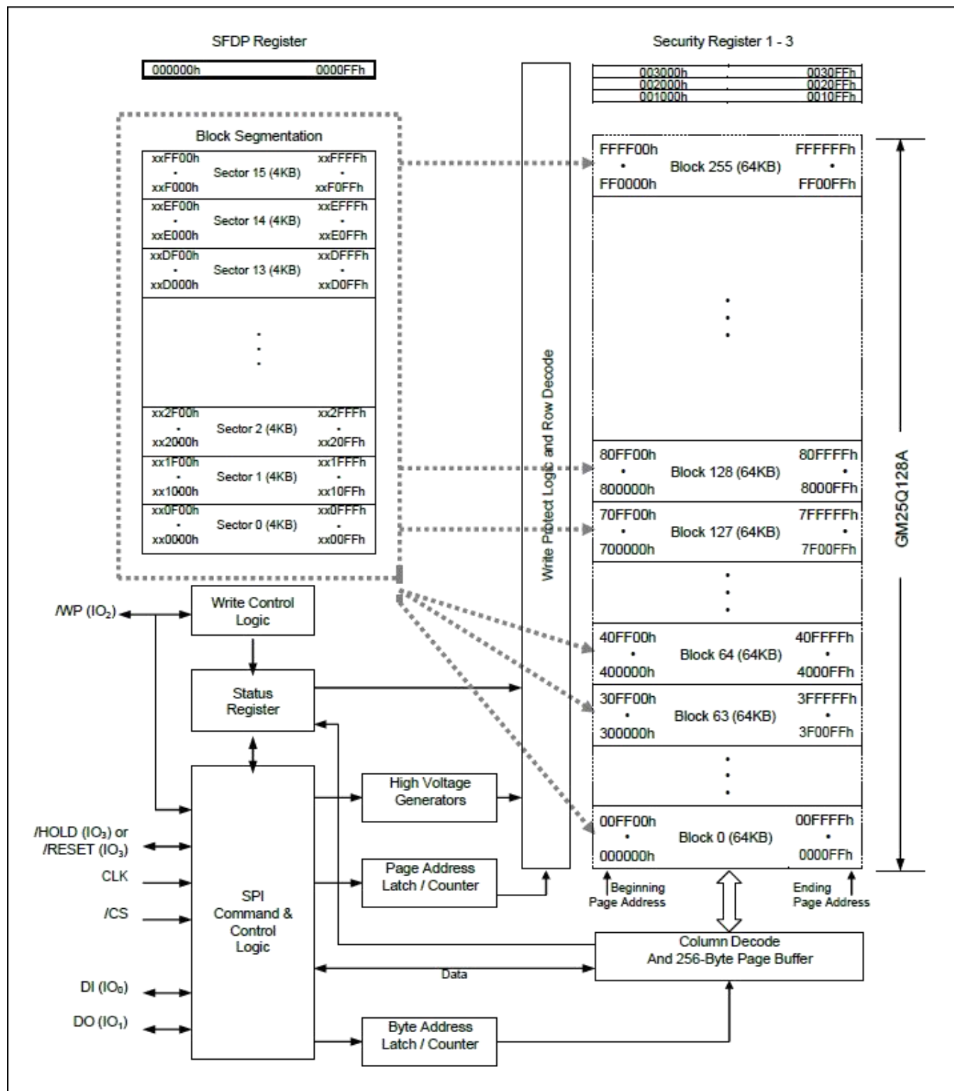
Figure 2. UD25Q128A Serial Flash Memory Block Diagram
