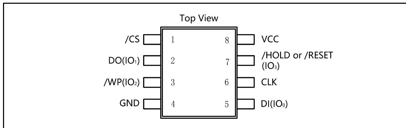
Figure 1a. UD25Q128A Pin Assignments, 8-pin SOIC 208-mil (Package Code S)
