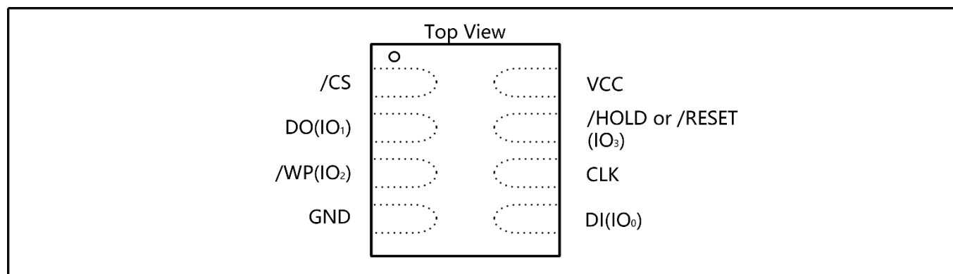
Figure 1b. UD25Q128A Pad Assignments, 8-pad WSON 6x5-mm/ 8x6-mm (Package Code P/E)
