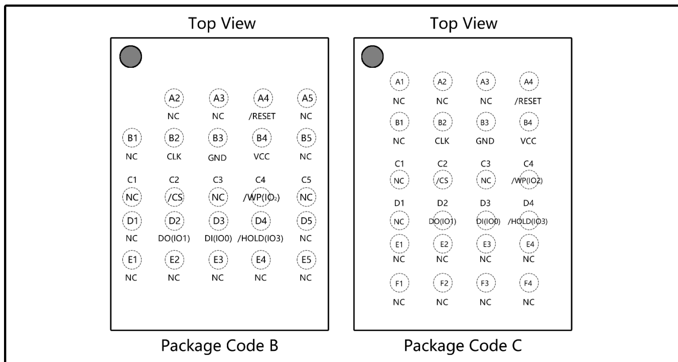
Figure 1d. UD25Q128A Ball Assignments, 24-ball TFBGA 8x6-mm (Package Code B/C)
