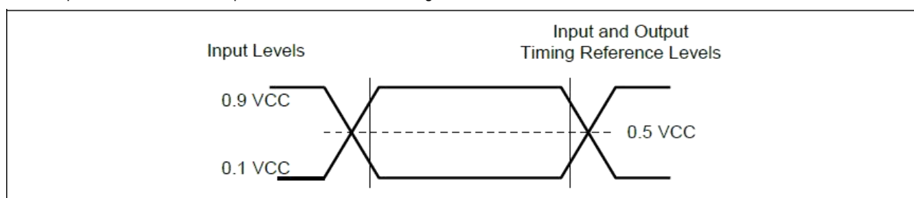
Figure 37. AC Measurement I/O Waveform
