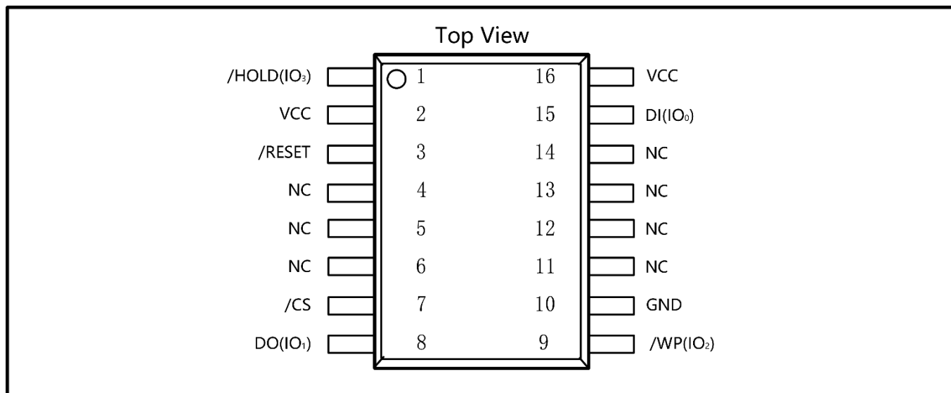
Figure 1c. UD25Q128A Pin Assignments, 16-pin SOIC 300-mil (Package Code F)
