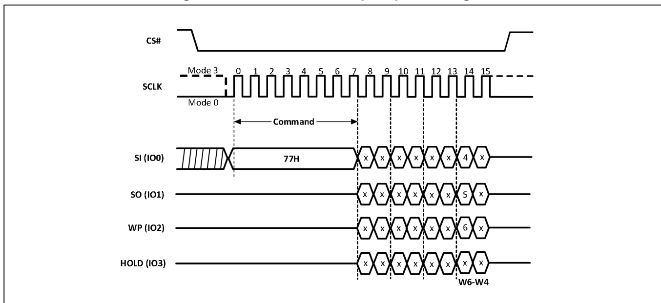
Figure-16. Set Burst with Wrap Sequence Diagram
