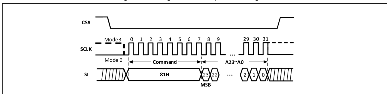
Figure-17. Page Erase Sequence Diagram
