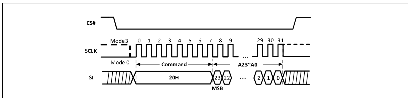
Figure-18. Sector Erase Sequence Diagram
