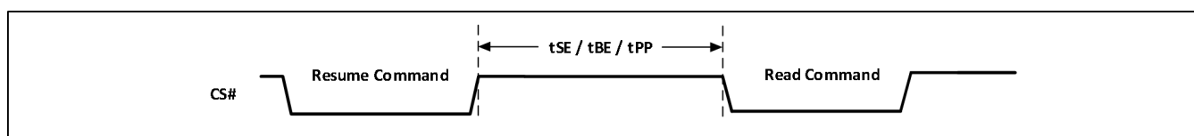
Figure-39. Program Resume and Erase Resume Sequence Diagram
