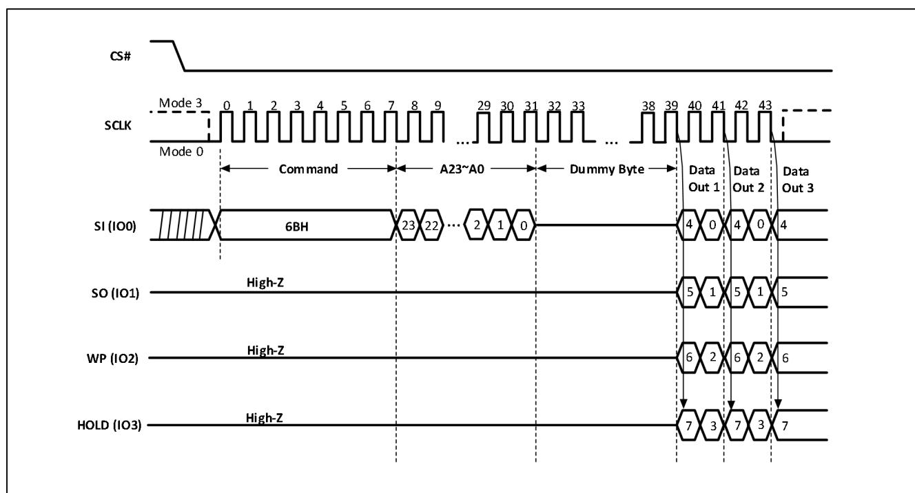
Figure-14. Quad Output Fast Read Sequence Diagram
