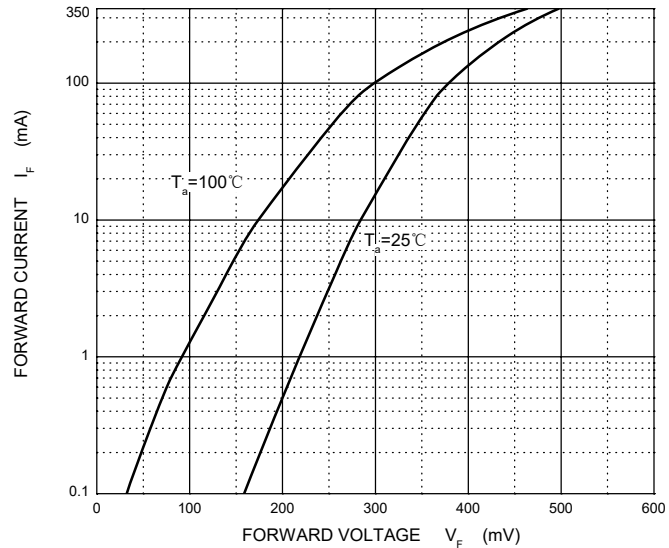
Forward Characteristics
