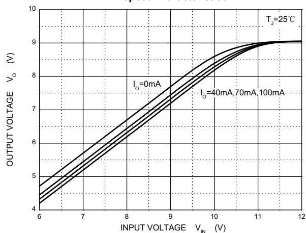
Dropout Characteristics
