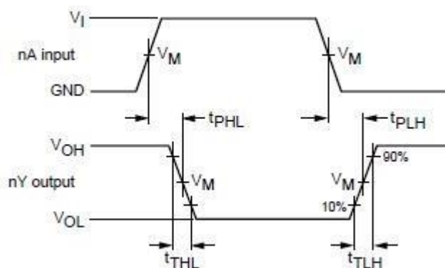
Fig.6 The input (nA) to output (nY) propagation delays and output transitions times.
