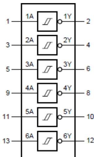
Fig.1 Logic symbol
