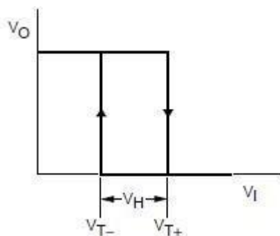
Fig.4 Transfer characteristic
