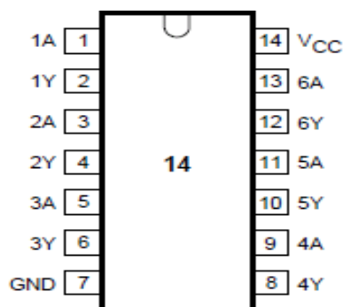
Fig.3 Pin configuration
