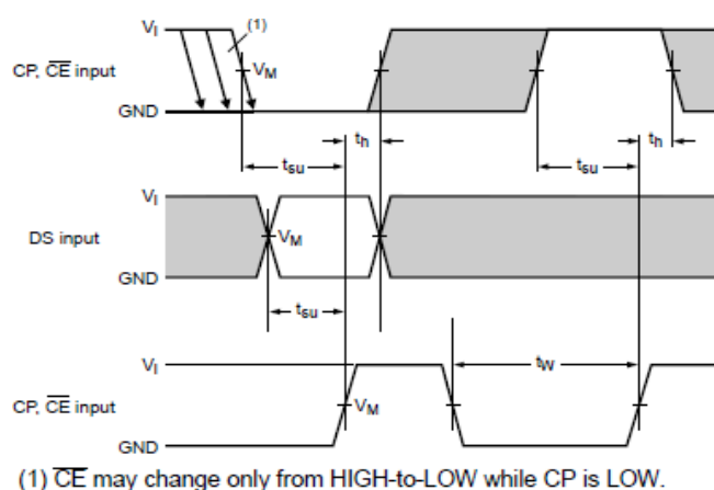
Figure 9. The set-up and hold times from the serial data input (DS) to the clock (CP) and clock enable (CE) inputs, from the clock enable input (CE) to the clock input (CP) and from the clock input (CP) to the clock enable input (CE)
