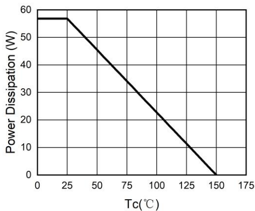
Figure 3. Power Dissipation
